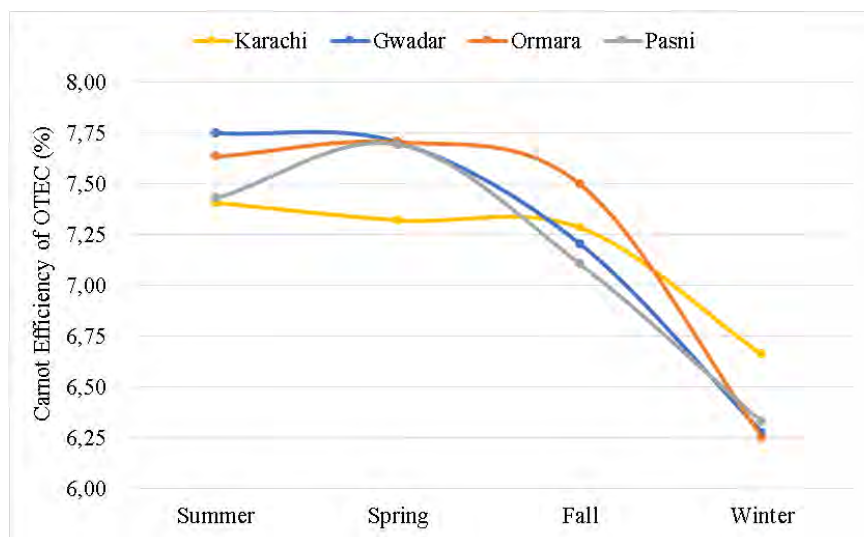
FIG. 18 Seasonal variations in Carnot efficiency of OTEC at 1500 m depth.
