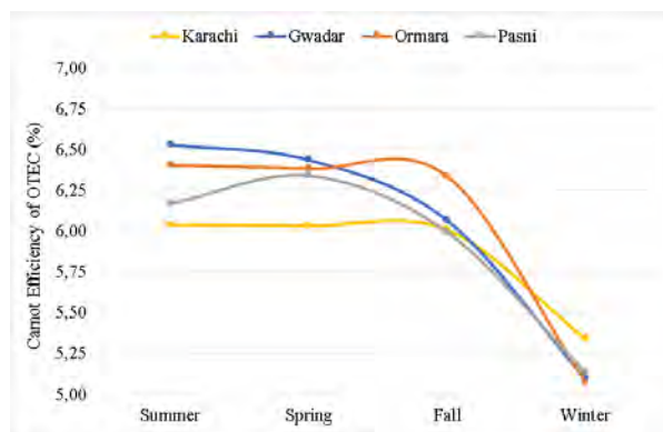
FIG. 16 Seasonal variations in Carnot efficiency of OTEC at 1000 m depth.
