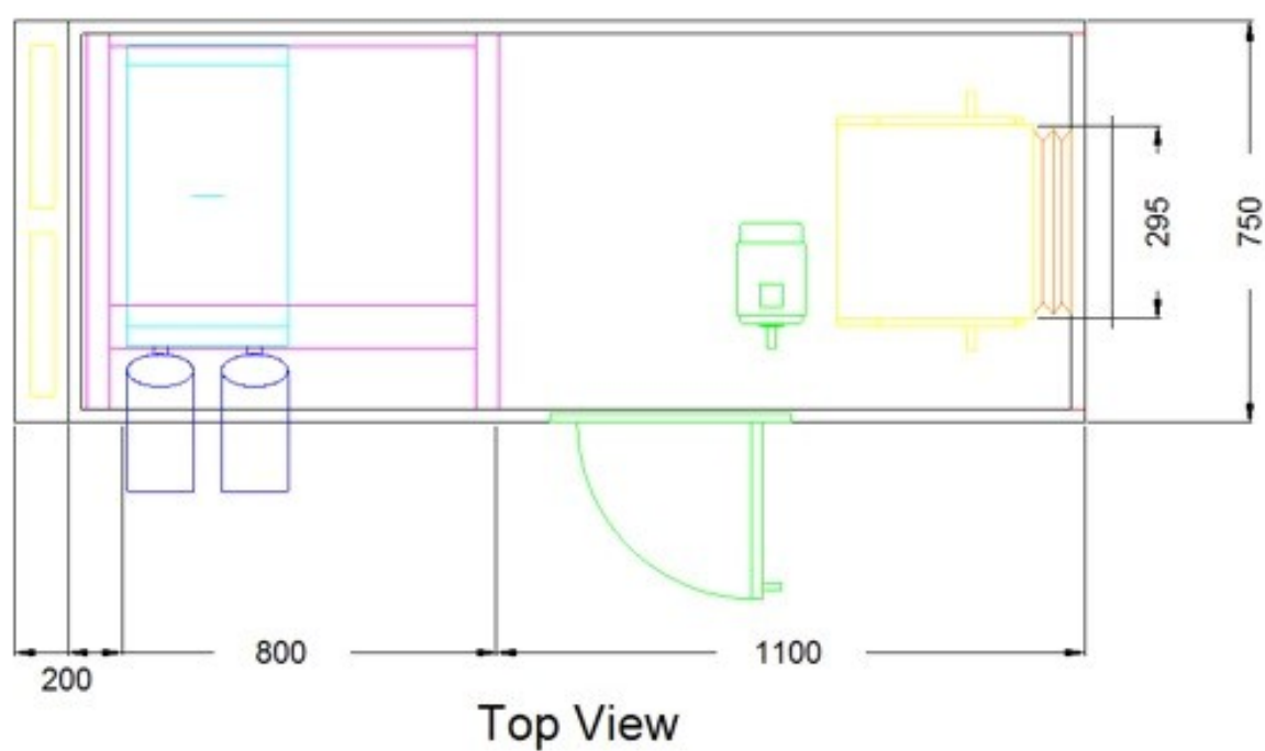
FIG. 10 2D design of AHU
