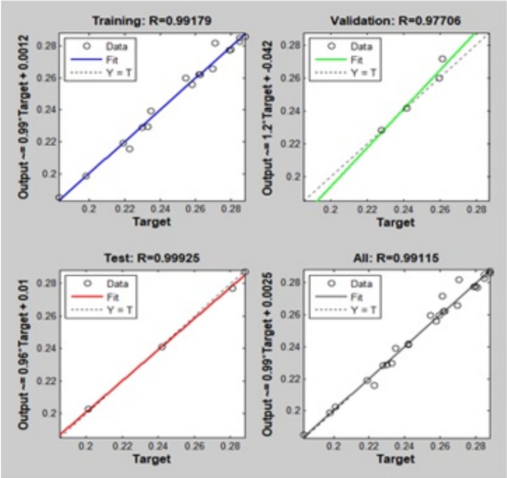
FIG. 5 Performance of ANN
