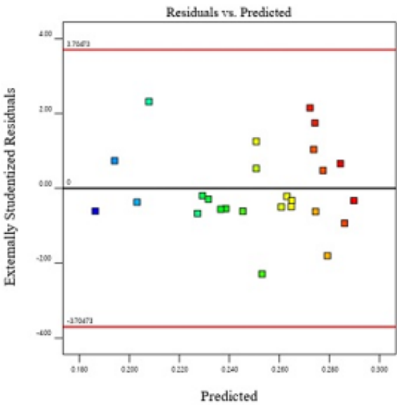
Figure 2 (b) Residual vs. Expected relationship
